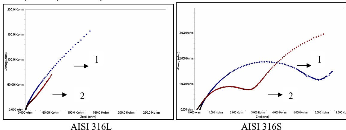
Figure3. The Nyquist curves of AISI 316L and AISI 316S alloy in artificial saliva, pH=6, at 37,2 °C and different time exposes and natural aeration conditions; (1), t=0 hours, (2), t=120 hours.
