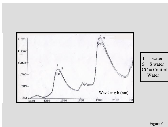
Figure 6. Infrared reflectivity spectrum of one emulsion. Reflectivity (R) was measured for one emulsion prepared with three types of water, and \log(1/R) is plotted versus wavelength. I: emulsion in I water, S: emulsion in S water, CC: emulsion in distilled water.
