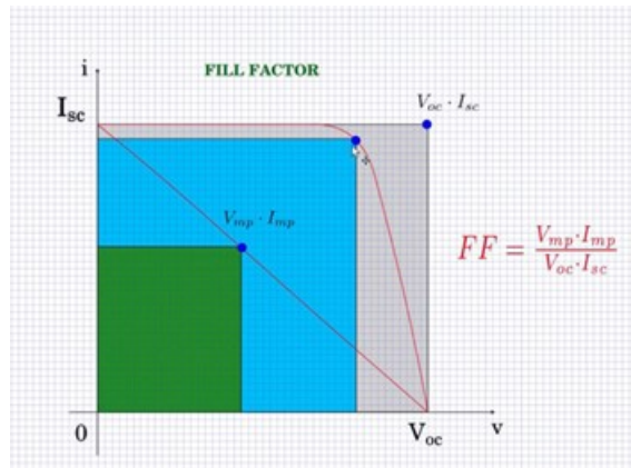
Fig.4. Fillfactor curve of solar PV cell
