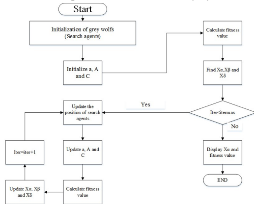
Fig 7 GWO Algorithm for MPPT
