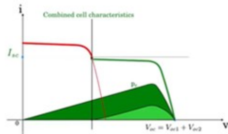
Fig.6. Improving solar efficiency by putting bypass diode
