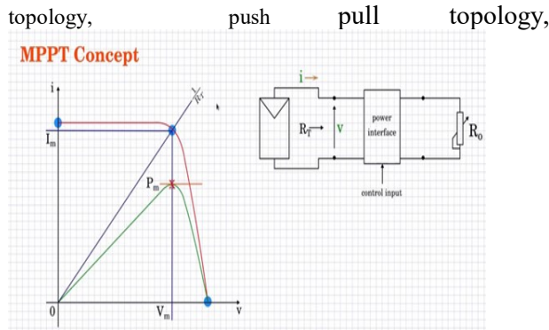
Figure3 MPPT for solar power output.
