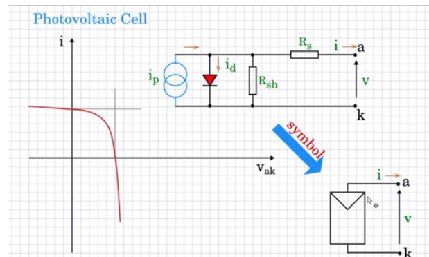
Fig.1. Practical solar cell.
