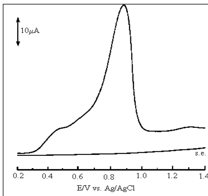
Figure 2. Square wave voltammogram of a glassy carbon disc electrode (1 mm diameter) containing 3 \text{mg ml}^{-1} dsDNA and 3 \mu\text{l} of a solution containing 4.5 \times 10^{-3} M of MTX on its surface, after being dried for 48 h. Supporting electrolyte 0.1 M acetate buffer pH 4.5. Frequency 50 Hz.
