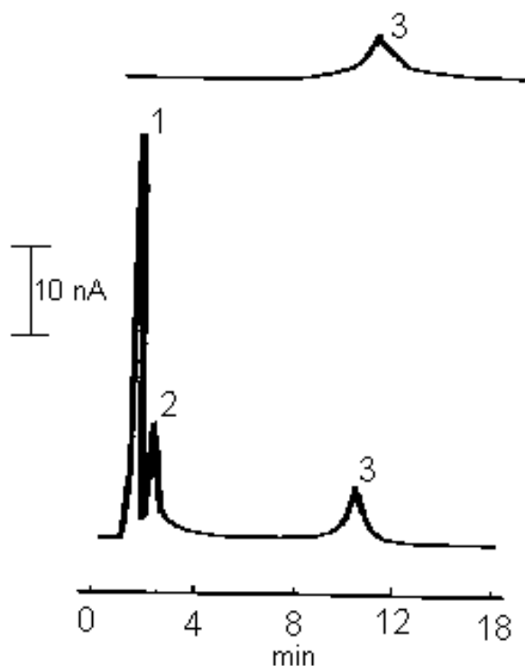
Figure 5. Chromatogram of a mixture of: (1) 2.0 mM L-cysteine, (2) 2.0 mM glutathione, (3) 0.50 mM 2ThU (1:1:1v/v/v): (A) electrochemical detection at a polyCoPC-CME at +0.75 V vs. Ag/AgCl and (B) u.v. detection at 280 nm.
