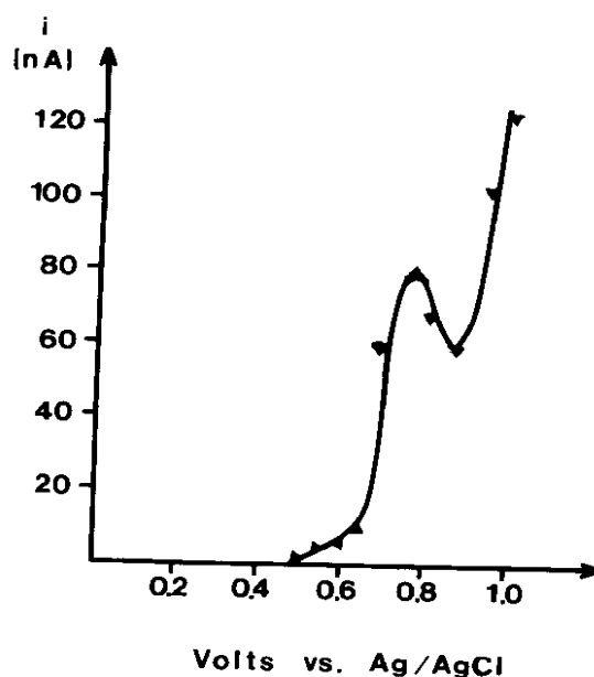
Figure 4. HDV of 2 ThU at polyCoPC-CME. Mobile phase was 5% CH 3 CN/95% 0.050 M phosphate buffer (pH, 3.0).
