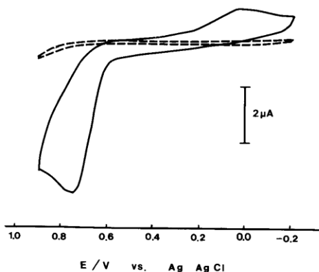
Figure 1. Cyclic voltammogram obtained for 0.5 mM 2 ThU in 0.050 M phosphate buffer (pH=3.0) at polyCoPC-CME. Shown as a dashed line is the voltammogram obtain at an unmodified electrode. Scan rate, 50 mV/s.
