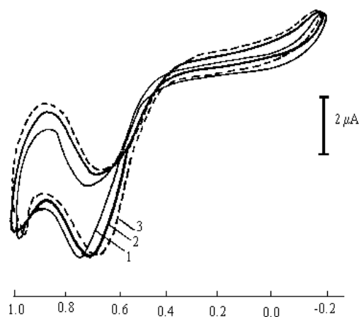
Figure 3. Influence of pH upon potential. (1) pH=2.5, (2) pH=5.5, (3) pH=8.0.
