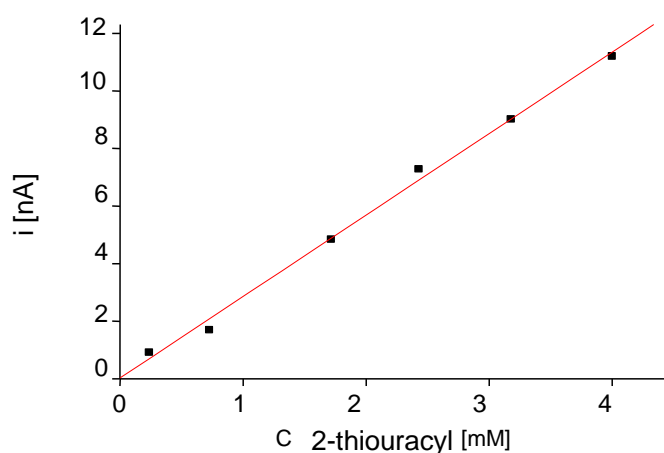
Figure 2. Calibration graph for 2 ThU.
